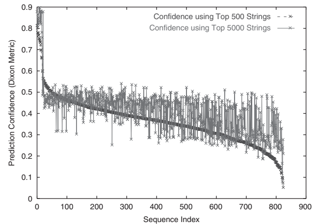
Fig. 4. The prediction confidence values using the top 5000 strings plotted on top of the order by using the top 500 strings. Only one prediction using the top 5000 strings remains not-so-confident. Colour version of this figure is available as Supplementary material online.
