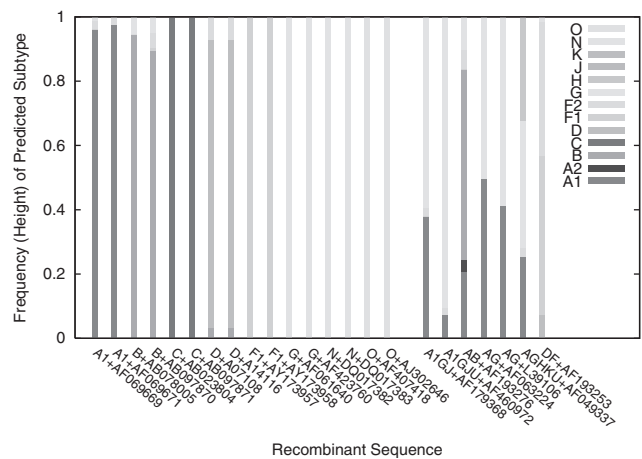
Fig. 6. The frequencies of the predicted subtypes for the 16 of 825 randomly selected pure subtype strains and the 7 recombinants, using the 5000 top ranked strings. Colour version of this figure is available as Supplementary material online.
