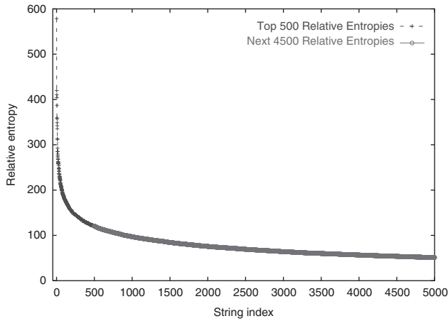
Fig. 1. The relative entropy scores of the 5000 top ranked strings, in decreasing order, in which the 500 top ones are colored blue. Colour version of this figure is available as Supplementary material online.
